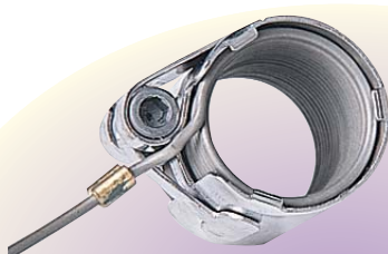
Cam Operated Clamping
